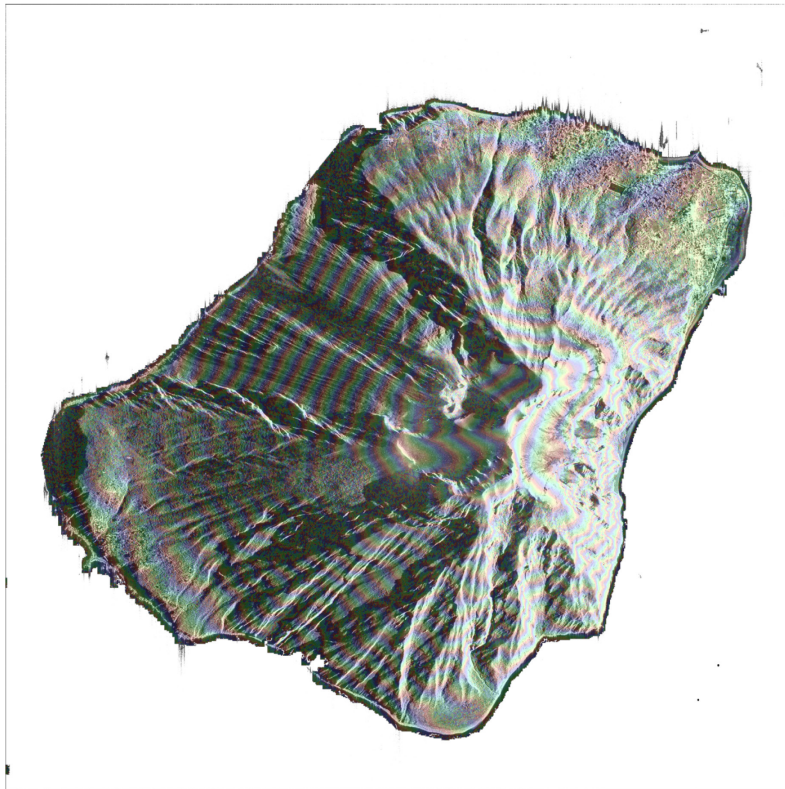
Figure 2: Overlay of the wrapped phase and amplitude SAR images over the Stromboli Island showing how the phase itself provide indication of the topography of the scene. The data has been acquired by the COSMO/SKYMED system.
