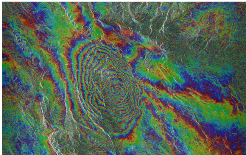
Figure 4: Differential interferogram associated with the main shock of April 6 th 2009 in the l'Aquila earthquake sequence: each fringe (change of color from blue to red) corresponds to a lowering of the surface area of about 2cm: the total subsidence is more than 20cm. Images were acquired by the COSMO/SKYMED constellation on 4 th and 12 th of April 2009.
